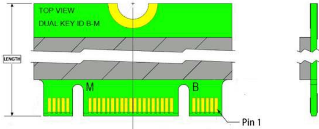
Figure 3-1 Pin Connectors
