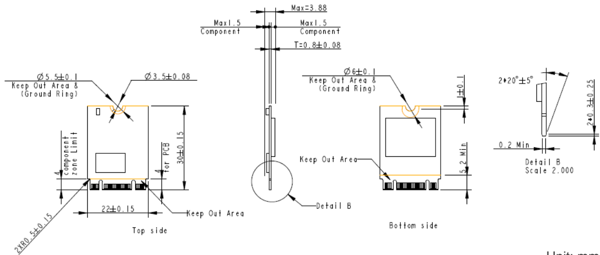
Figure 10-1 Dimensions
