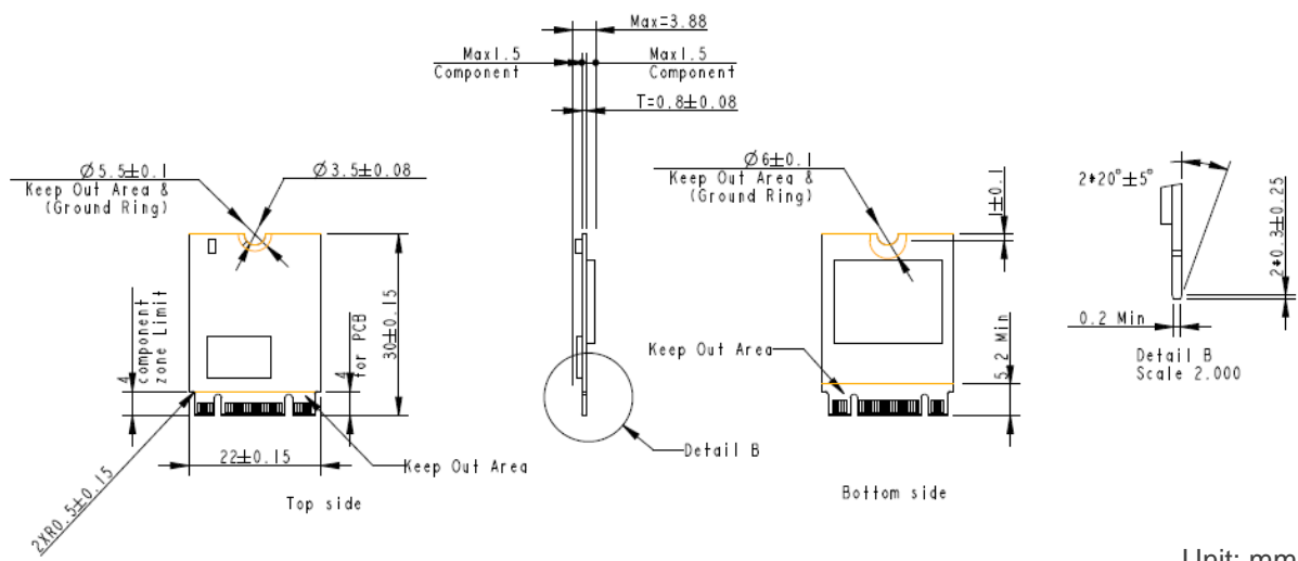
Figure 10-1 Dimensions
