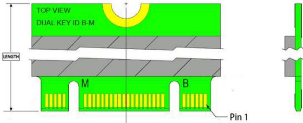
Figure 3-1 Pin Connectors
