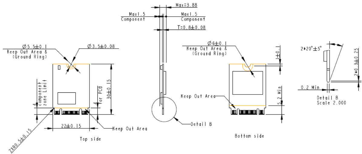
Figure 10-1 Physical Dimensions
