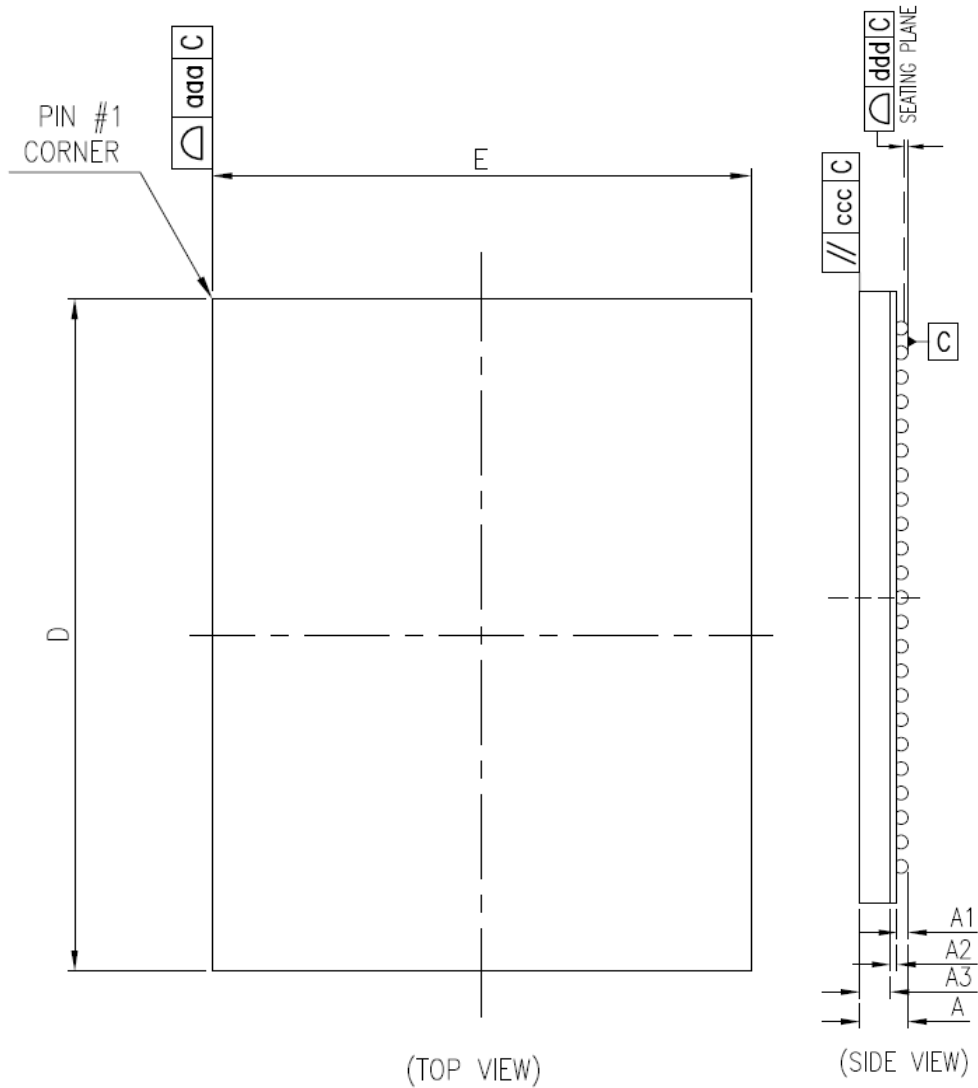
Figure 10-1 Physical Dimensions
