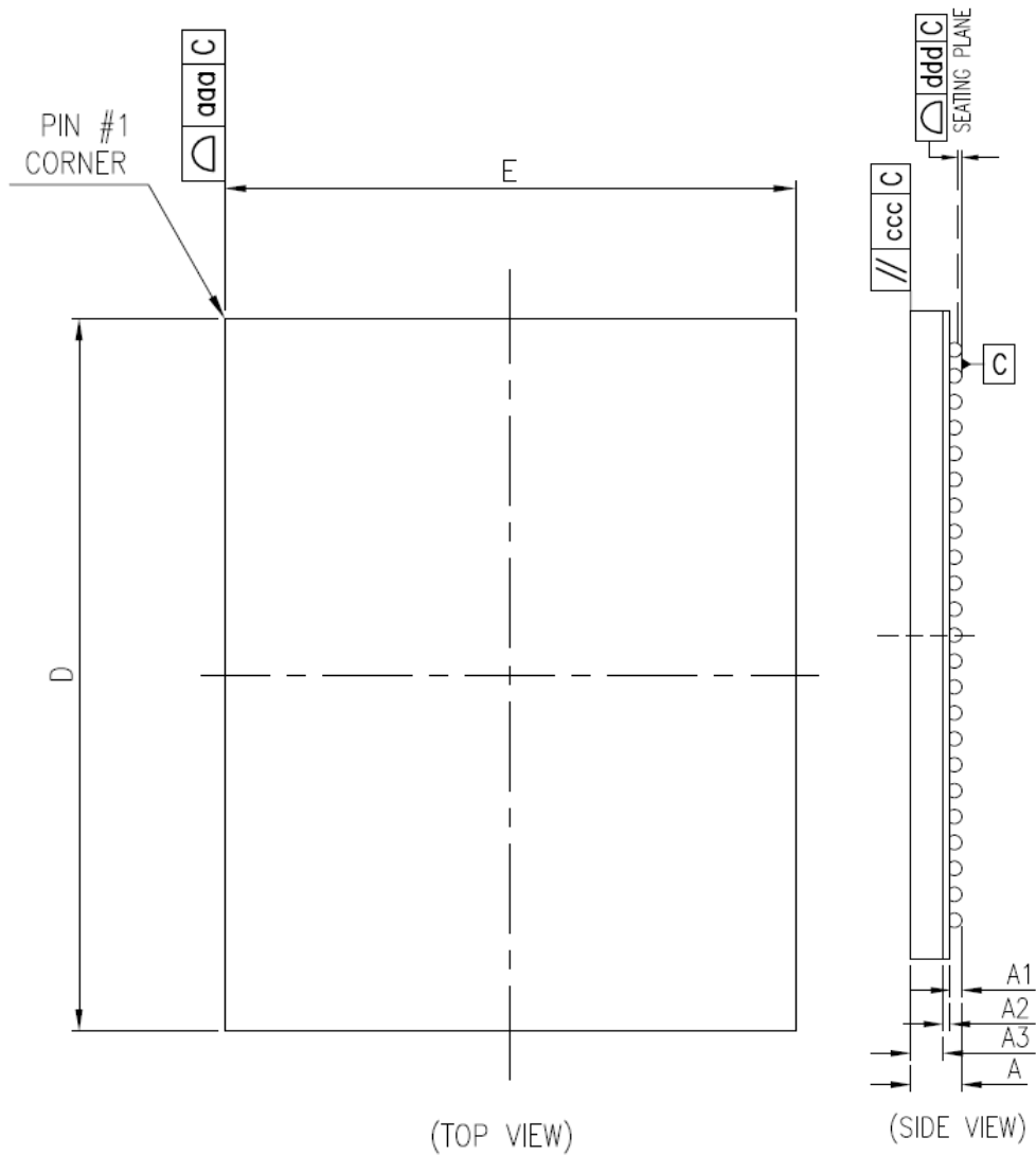
Figure 10-1 Physical Dimensions
