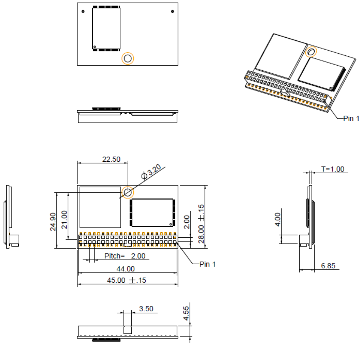
Figure 8-1 Dimensions
