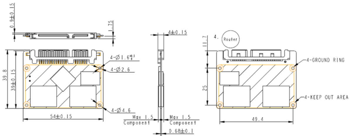
Figure 9-1 Physical Dimensions
