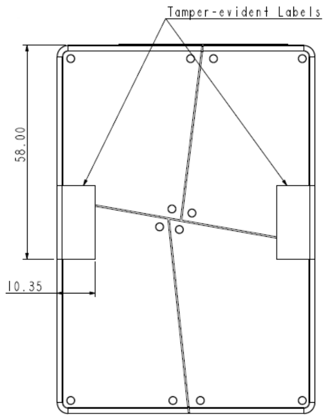
Figure 9-1 Physical Dimensions
