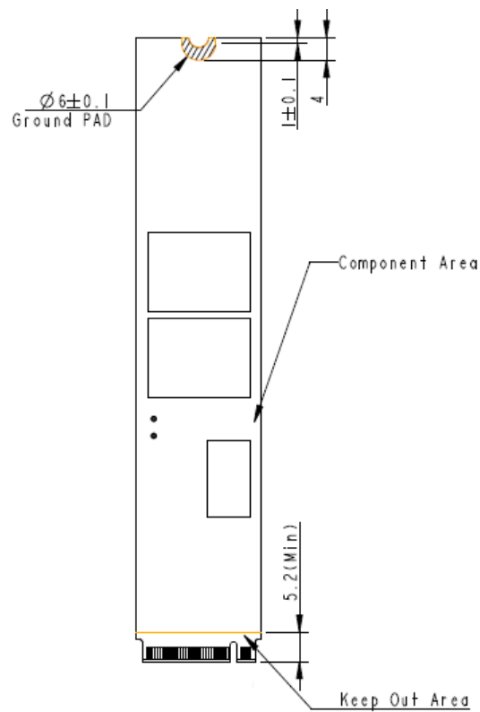
Figure 9-1 Physical Dimensions
