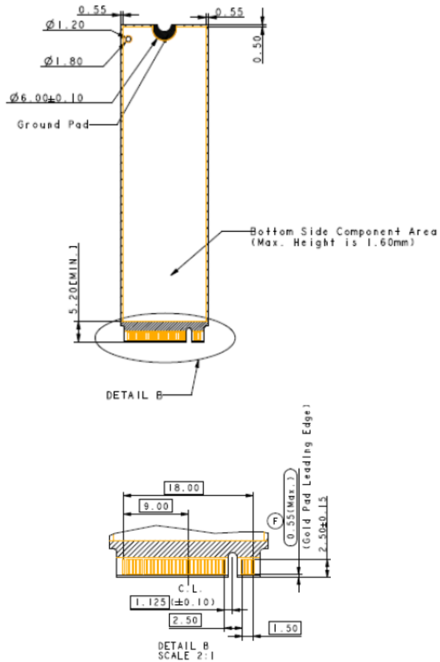
Figure 9-3 Dimensions – Bottom View
