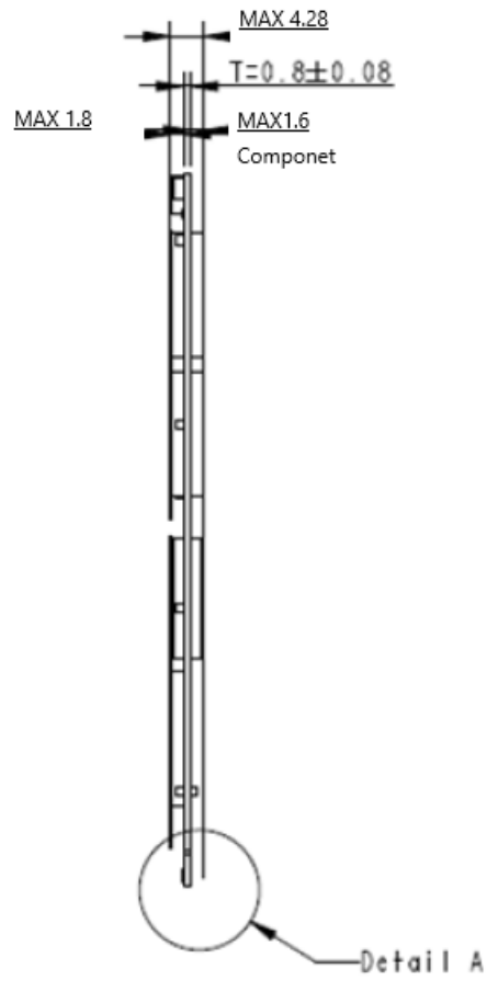
Figure 9-2 Dimensions – Side View
