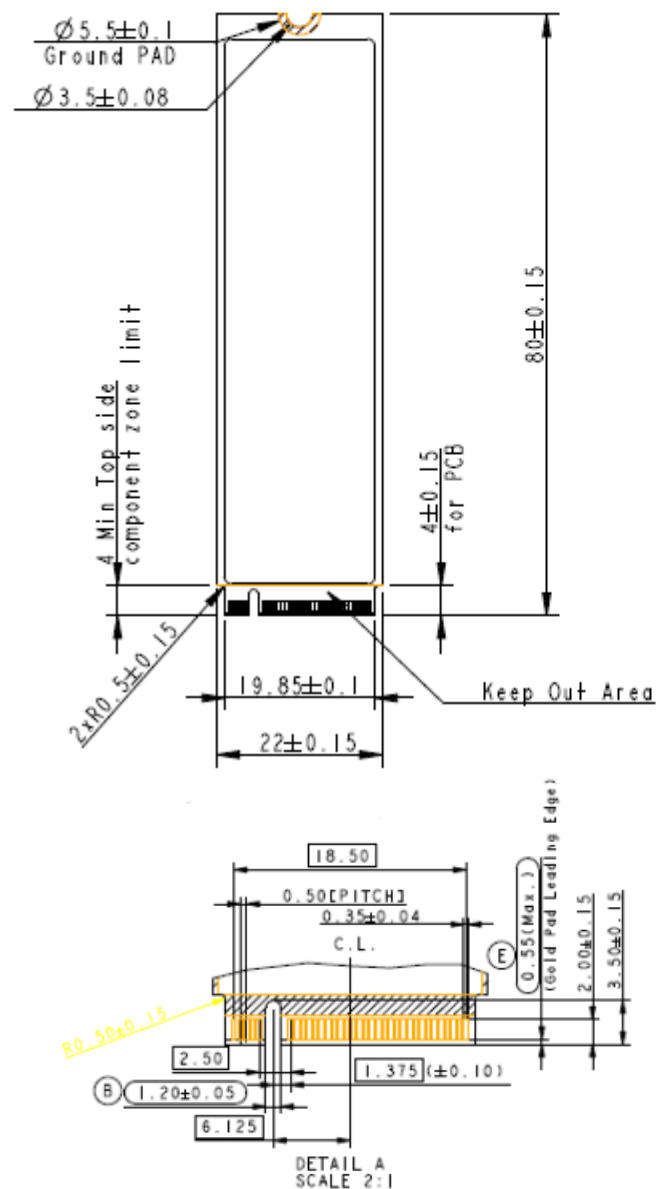
Figure 9-1 Dimensions – Top View
