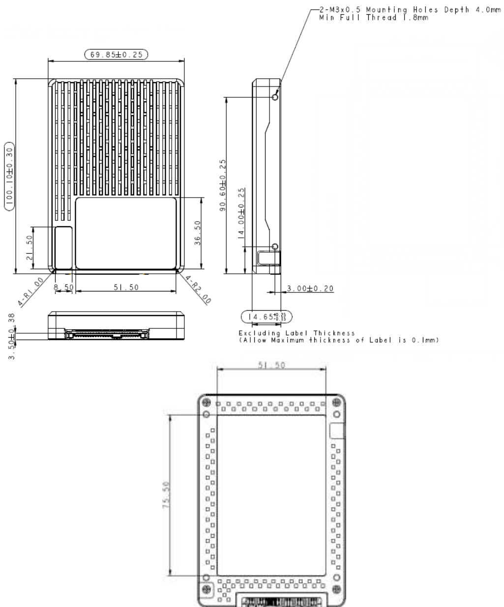
Figure 10-1 Physical Dimensions
