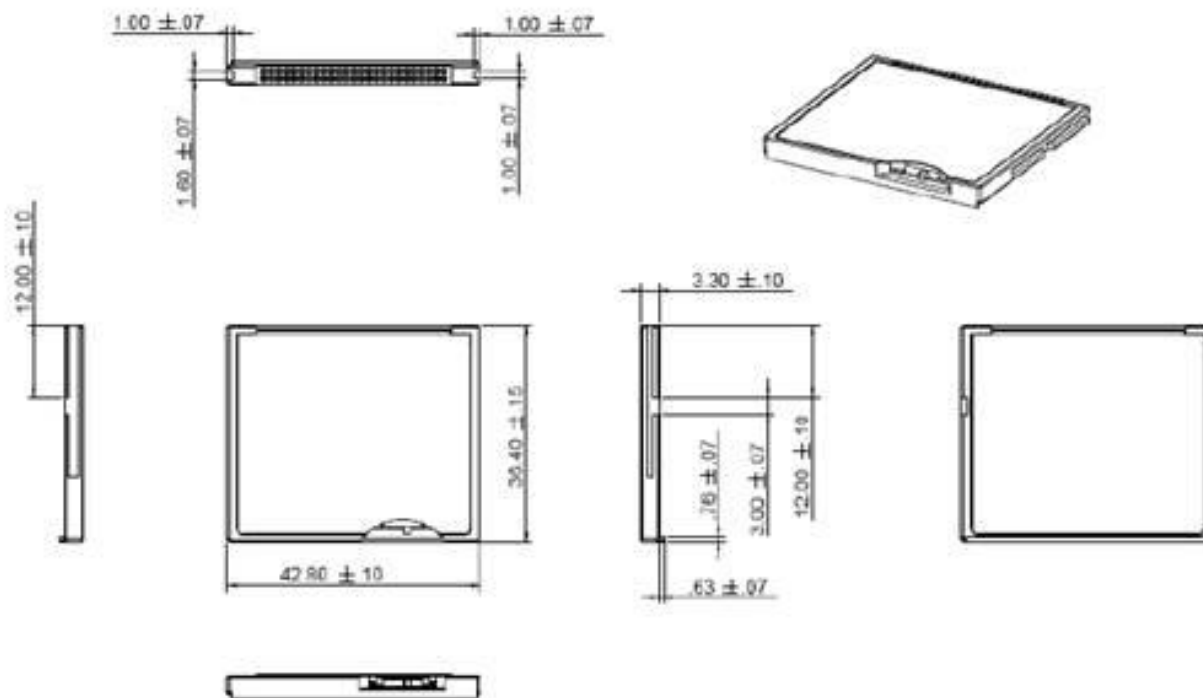
Figure 7-2 Physical Dimensions
