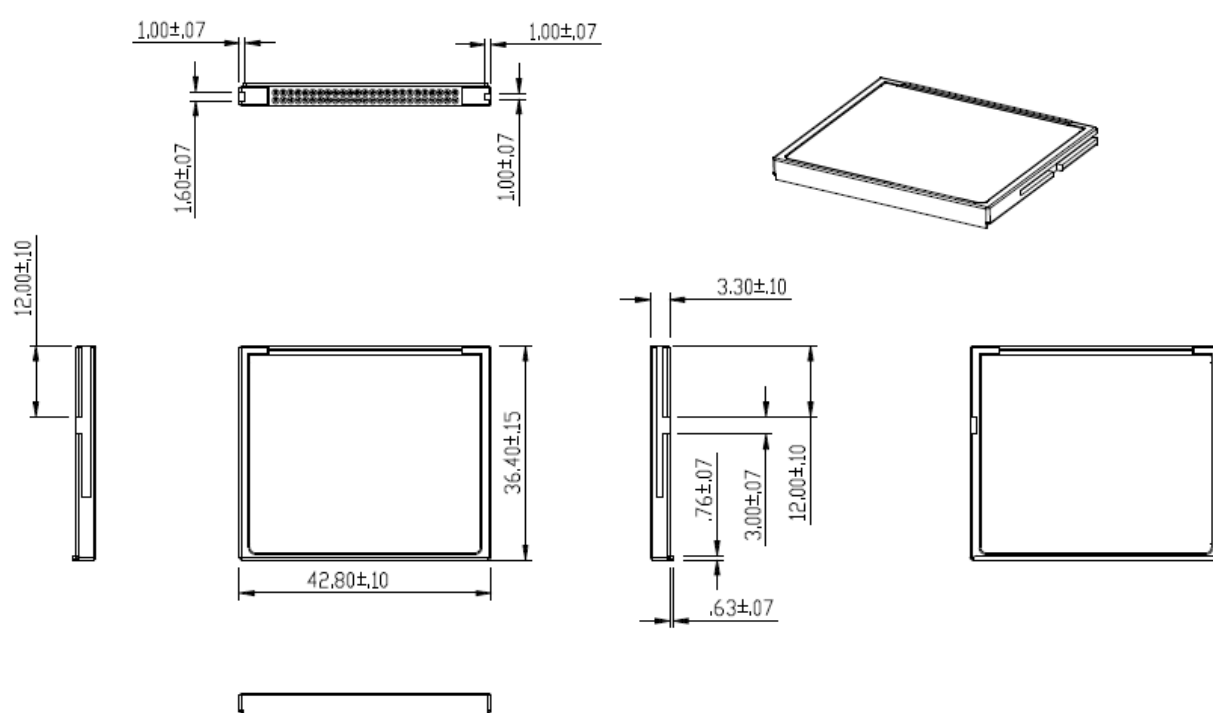
Figure 8-1 Physical Dimensions
