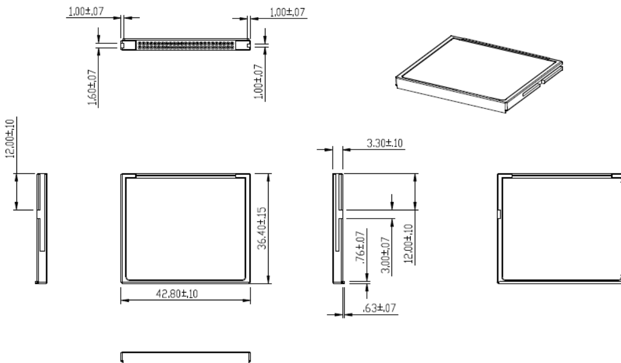
FIGURE 7-1: Physical dimension
