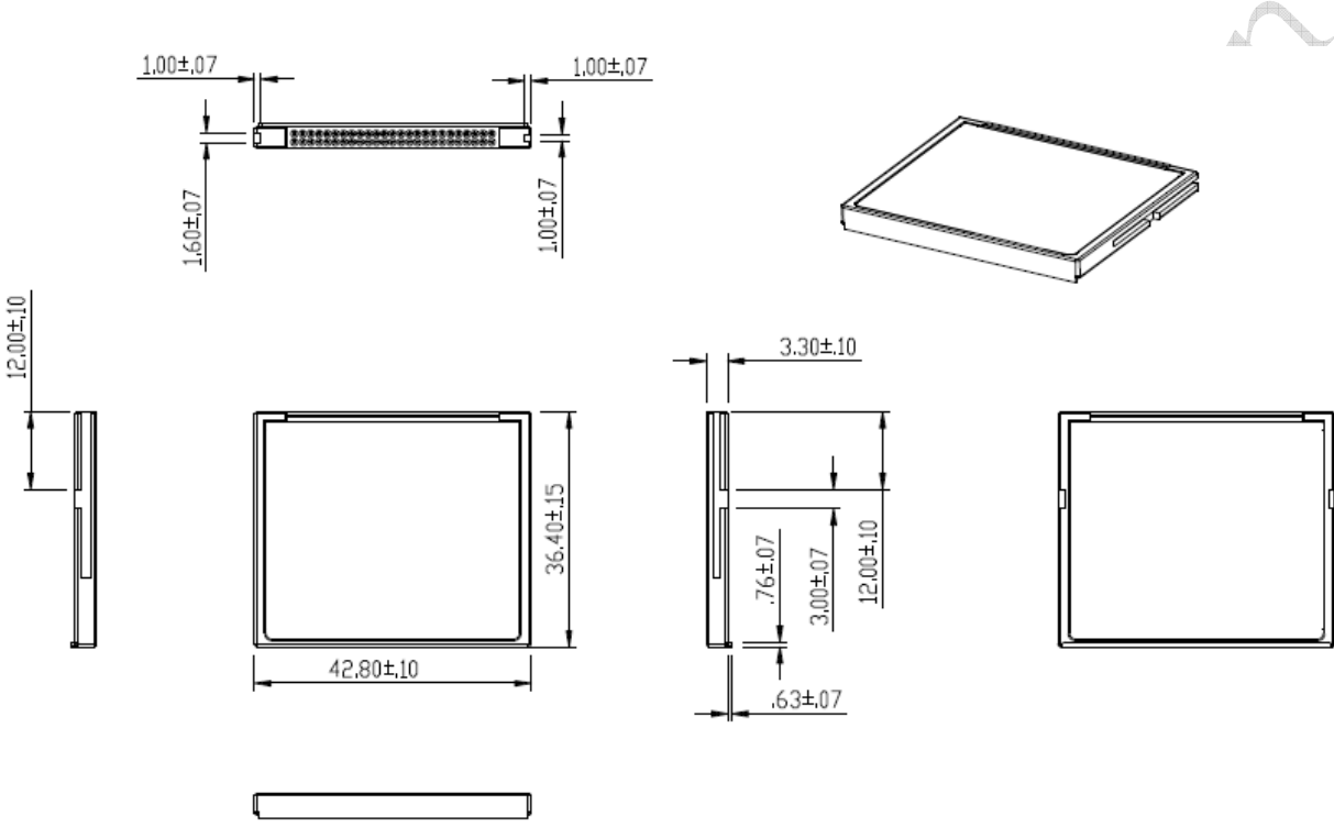
FIGURE 7-1: Physical dimension
