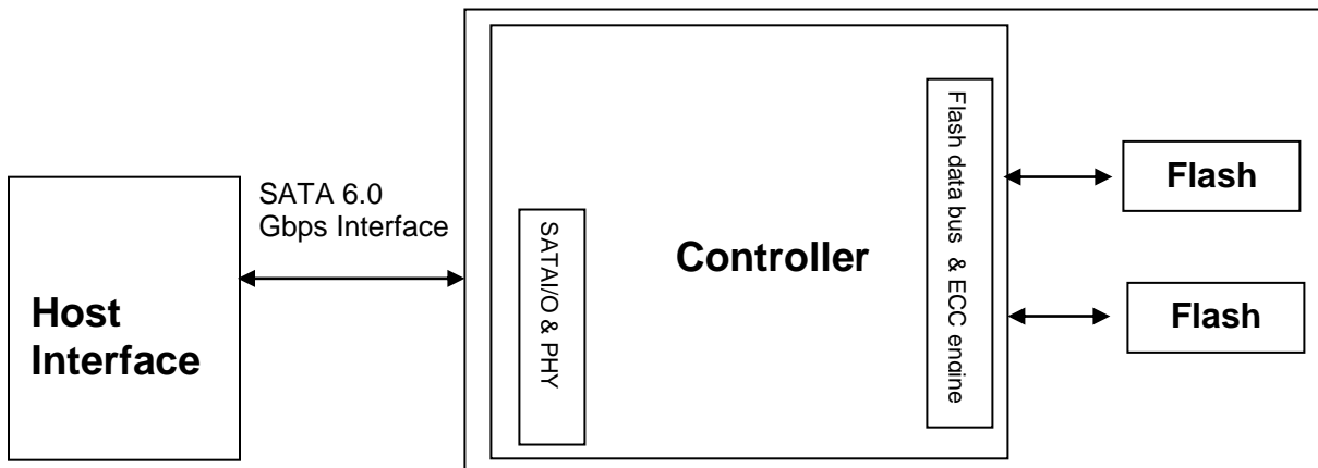
Figure 2-1 Apacer SM220-CFast Block Diagram
