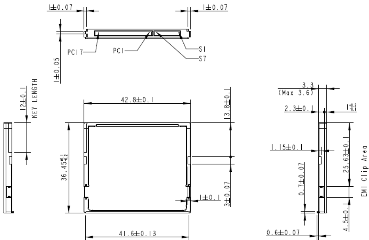
Figure 8-1 Physical Dimensions
