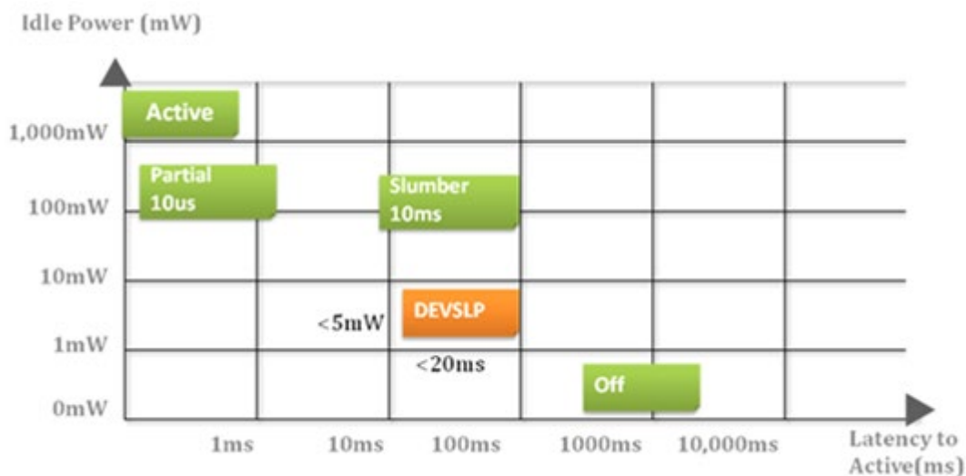
Figure 5-1 Device Sleep
