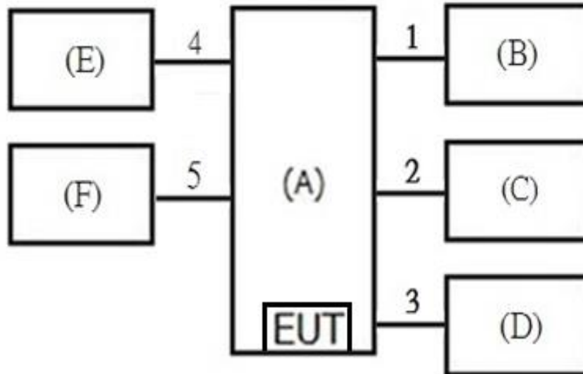
Test Setup Diagram - Radiated emission above 1GHz
