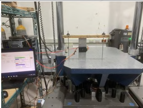
11. Operating Mechanical Shock Test (+Y axis)
