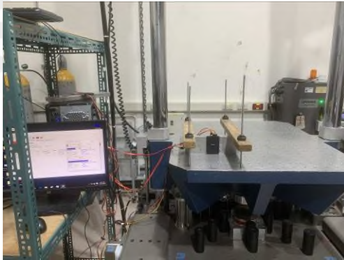
9. Operating Mechanical Shock Test (+X axis)
