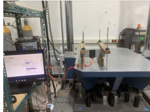
10. Operating Mechanical Shock Test (-X axis)
